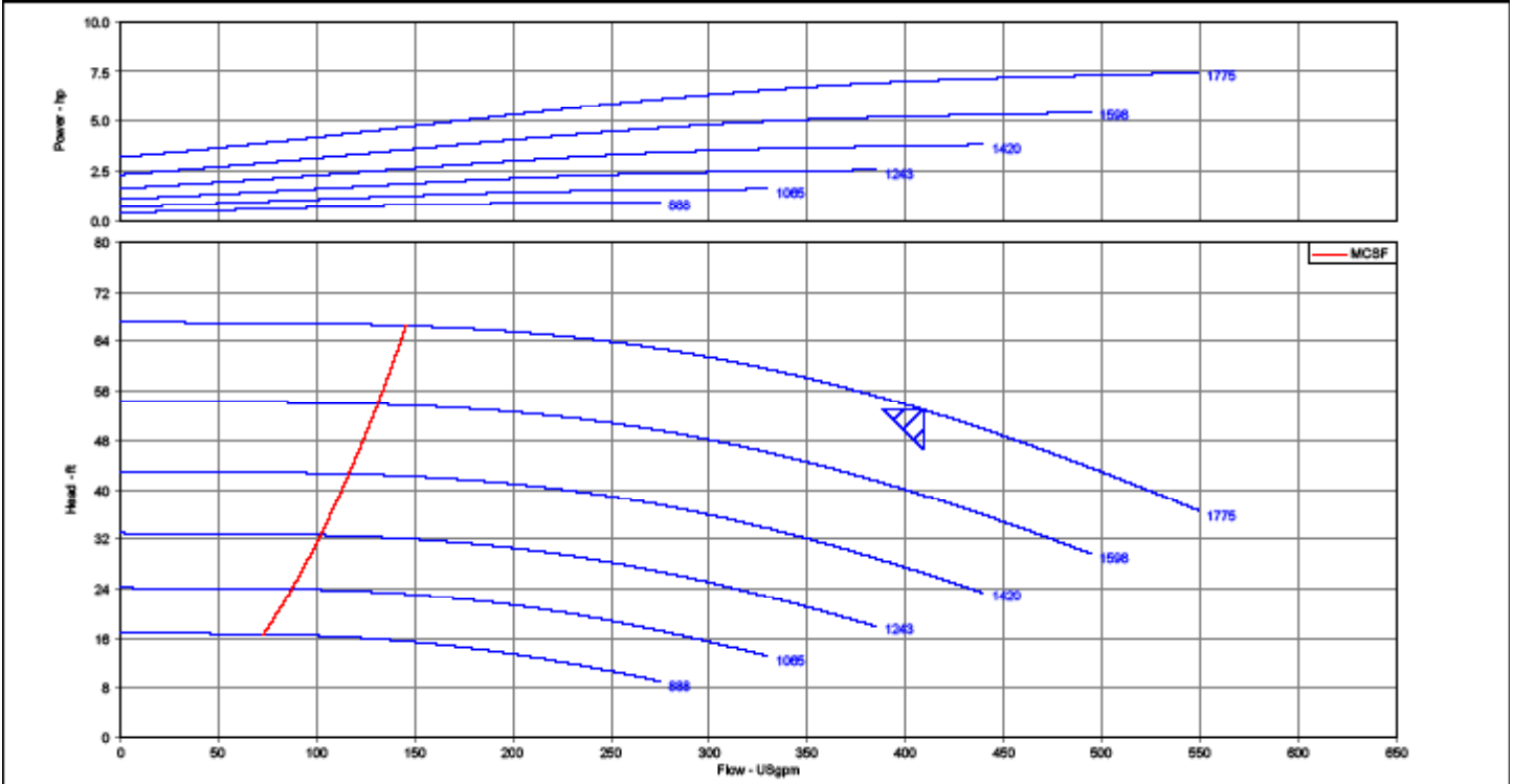
Multi-Speed Performance Curve
