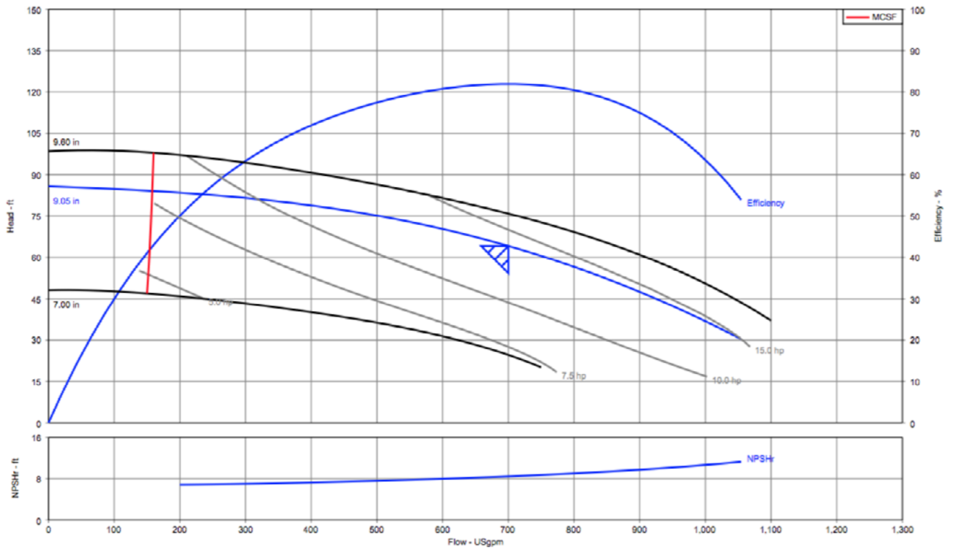
Pump Performance Curve
